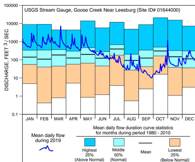
Figure 9. Stream discharge hydrograph for Goose Creek during 2019 compared to data from 1981-2010.
