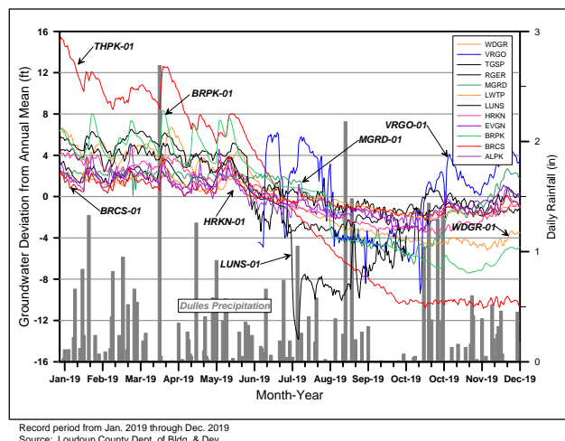
Figure 11. Groundwater level deviation at selected County monitoring wells.
