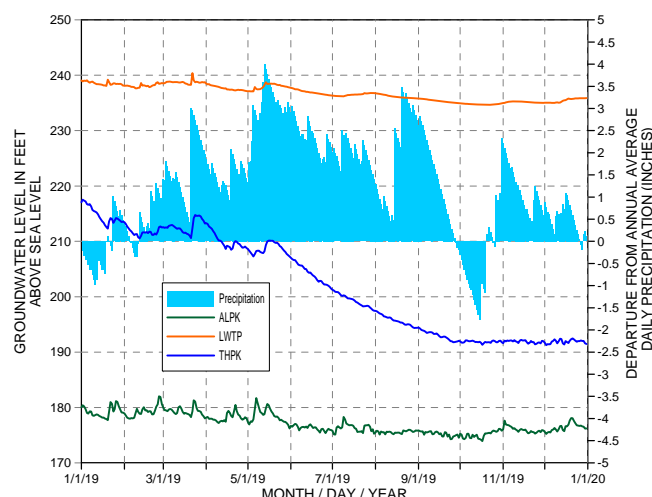
Figure 12. Groundwater hydrograph and daily rainfall in 2019.
